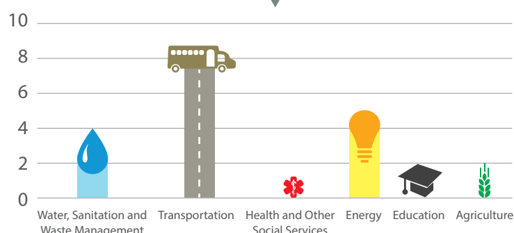
Figure II-4: Sector Distribution
